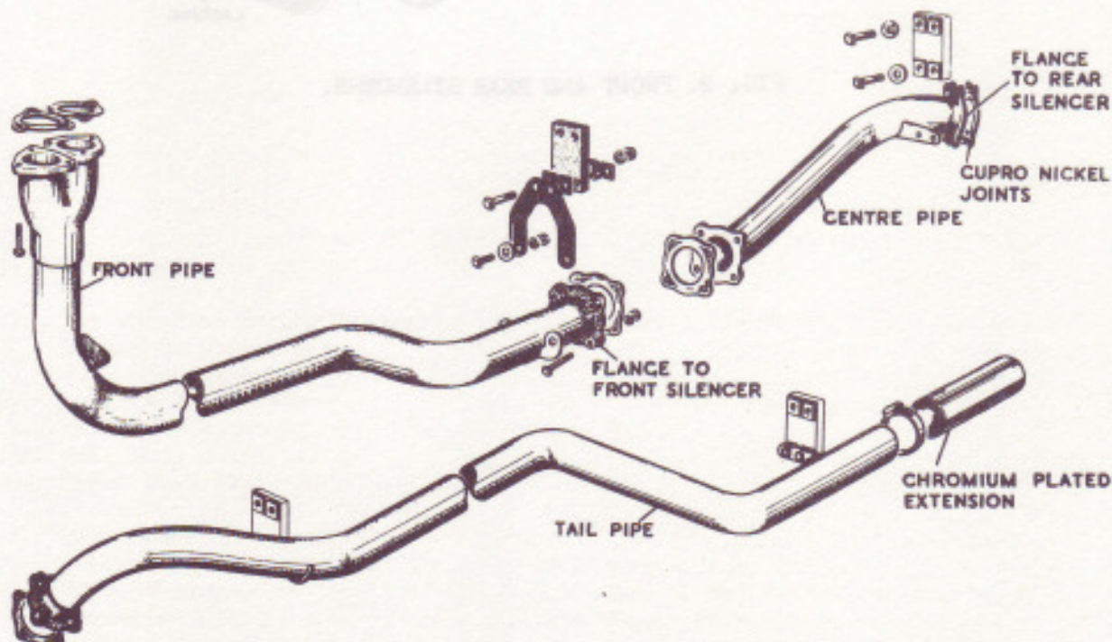
FIG. 1. EXHAUST PIPES
